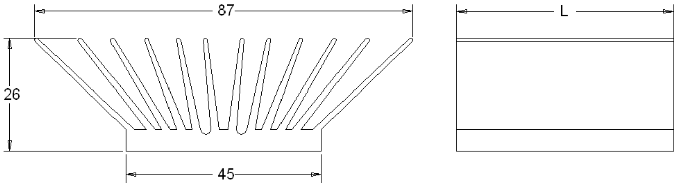
MECHANICAL OUTLINE (UNIT: MM)
